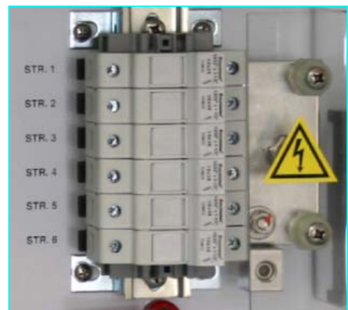
Finger-safe Fuse Holders
