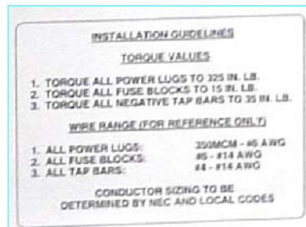
Silk-Screened Details
