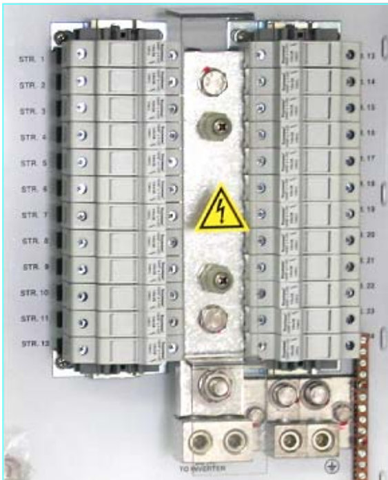
Finger-safe Fuse Holders Reinforced Busbars
